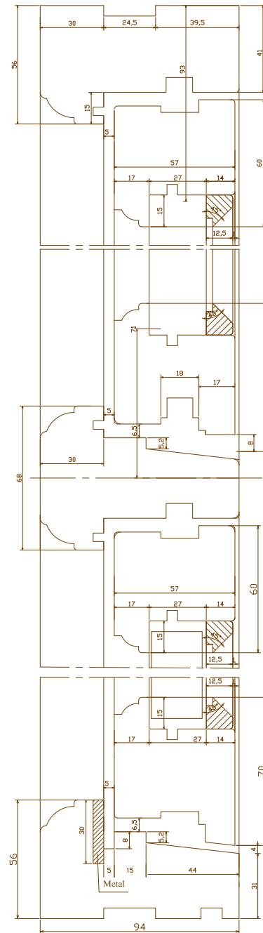
VERTICAL SECTION. OUTSIDE VIEW
