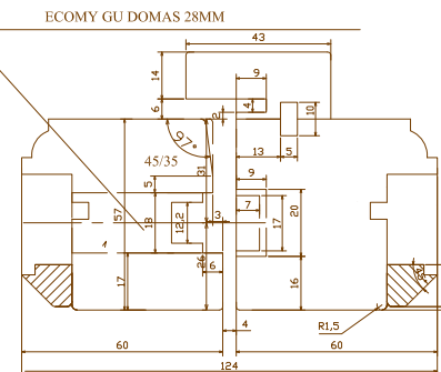
HORIZONTAL SECTION. OUTSIDE VIEW. BOTTOM SASH.
